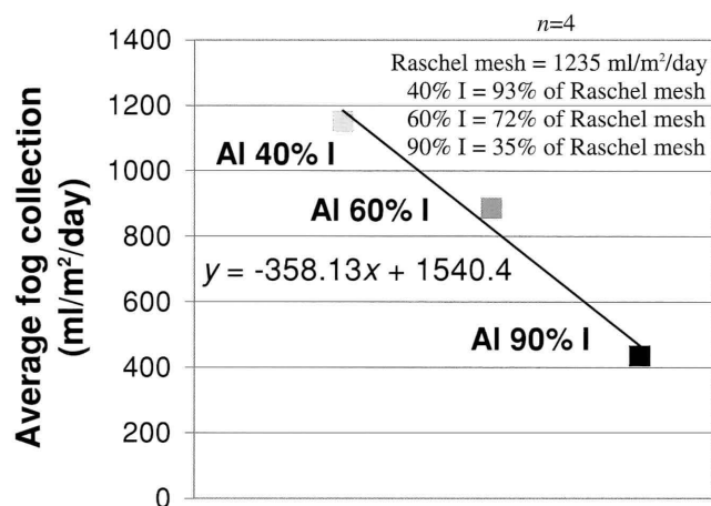
Figure 4 | Average fog collection in indoor aluminet collectors of varying percent shade coefficient.
