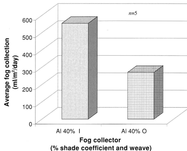
Figure 2 | Average fog collection in aluminet 40% collectors of indoor (I) and outdoor (O) weave.
